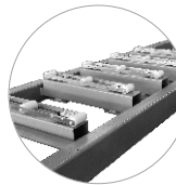
Abrasion resistant slip plates for 4 wheel alignment 四轮定位耐磨侧滑配置
